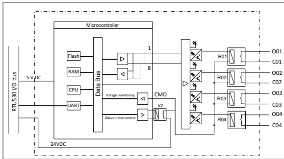
Figure 3: Block diagram binary output unit
